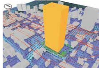
Air flow around the building
